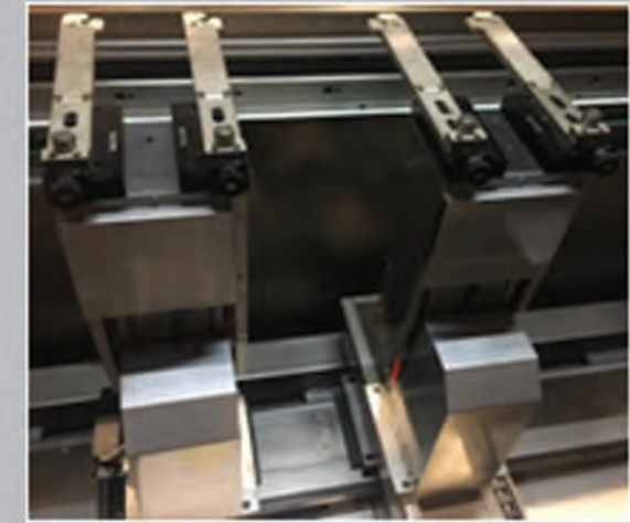
Optional multi-axis configurations: X1, X2, Z1, Z2, R1, R2 allow up to six different movements to be automatically calculated and set by the control
